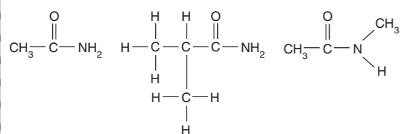
ethanamide 2-methylpropanamide N -methylethanamide
